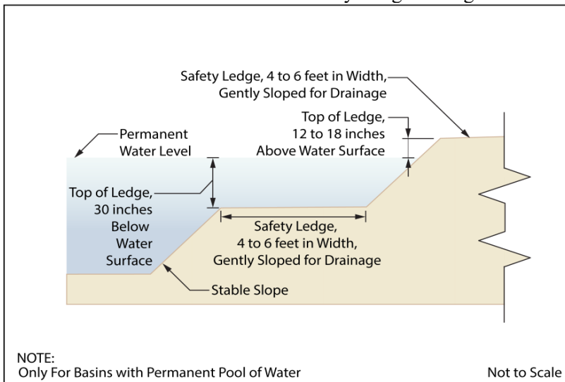
Elevation View –Basin Safety Ledge Configuration
